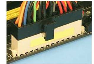
24-pin ATX power connector
